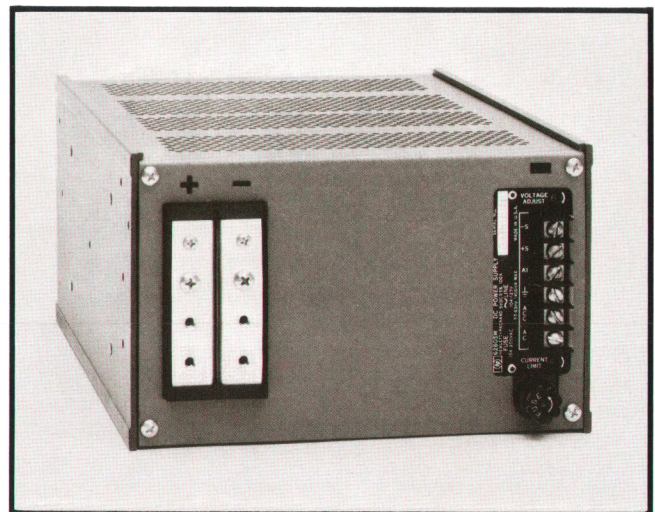
Fig. 1. Model 62605M Power Supply, designed for permanent installation, supplies current in a range from 0 to 100 A at 5 V. The switching regulator achieves 70% efficiency at full output.
