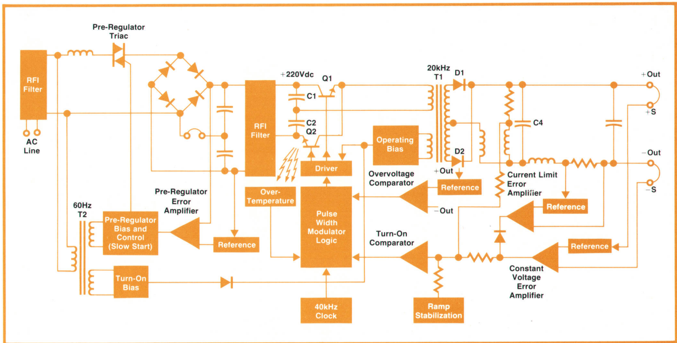
Fig. 2. Block diagram of the Model 62605M modular power supply. It operates directly from a 220V power line when the shorting strap is in place. With the strap removed (and some other minor changes), the input rectifiers no longer function as a bridge but become a voltage doubler that enables use on a 120V line.
