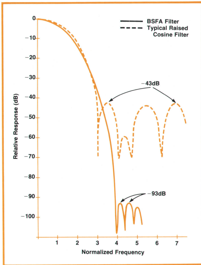
Fig. 6. BSFA digital filters have high out-of-band rejection, a primary requirement for BSFA. Here the BSFA filter frequency response is compared with a commonly used raised cosine filter. Note the 50 dB greater out-of-band rejection of the BSFA filter.
