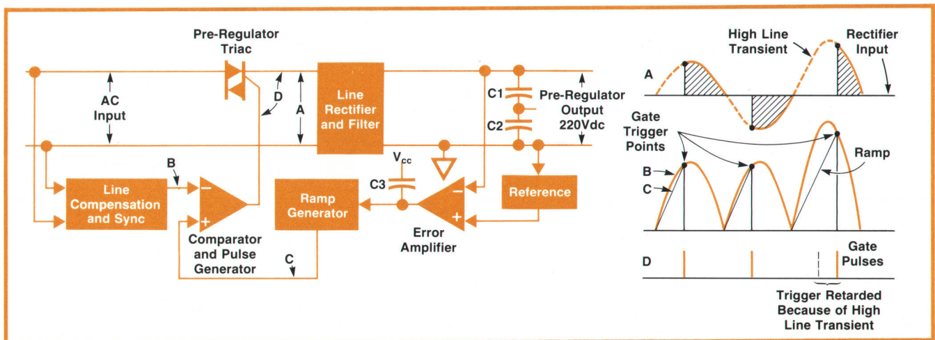
Fig. 5. Block diagram of the preregulator section. Operation is explained by the waveforms, which also show how the preregulator responds immediately to a change in line voltage.
