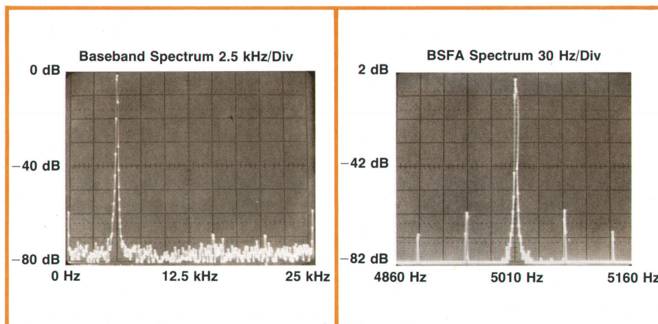
Fig. 1. The resolution and dynamic range improvements of band-selectable Fourier analysis (BSFA), a new capability of the 5451B Fourier Analyzer, are demonstrated by these power spectra of the output of a sine wave generator. The conventional baseband spectrum shows the 5-kHz fundamental and the third harmonic at -69 dB. The noise floor is 72 dB down. The BSFA spectrum shows that the fundamental is actually at 5010 Hz and that there are 60-Hz and 120-Hz sidebands. The noise floor is greater than 80 dB down.
