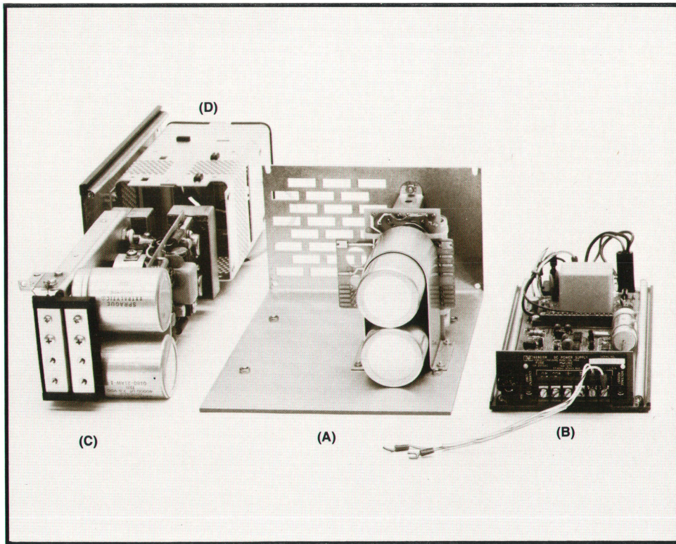
Fig. 4. Modular construction simplifies assembly and disassembly.
