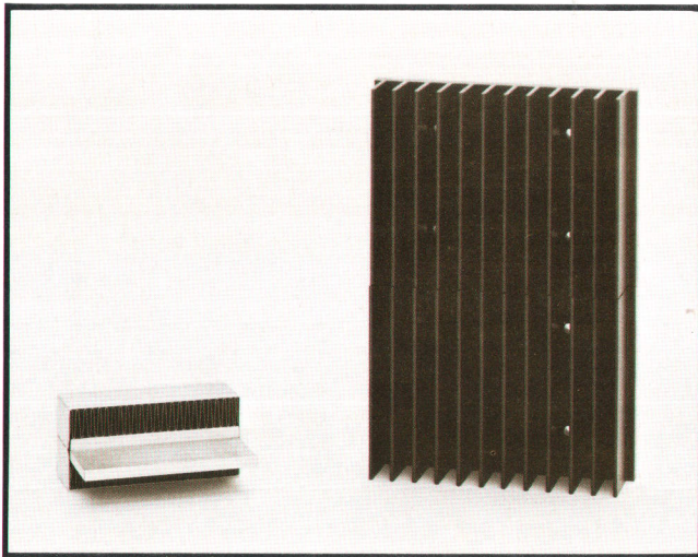
Fig. 3. Heat is removed from the power mesh through a heat exchanger (left) that rises in temperature only 0.5^{\circ}\text{C}/\text{W} with an air flow of 10\text{ ft}^3/\text{s} . An equivalent convection-cooled heat sink is shown on the right.
