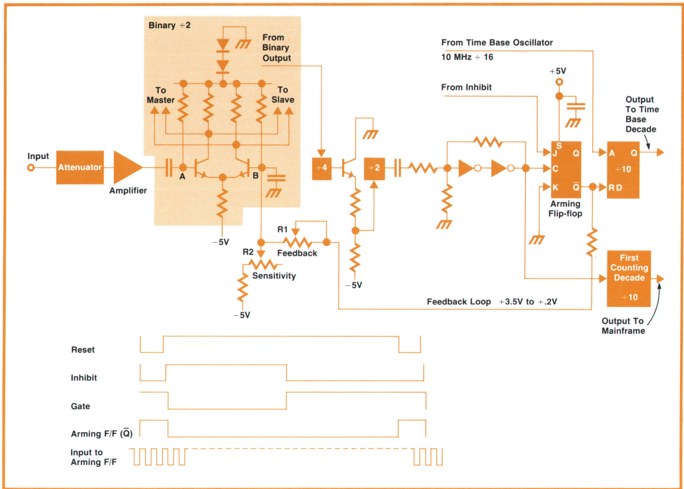
Fig. 8. Feedback loop reduces input sensitivity until a large enough input signal is present, then increases sensitivity during counting.
