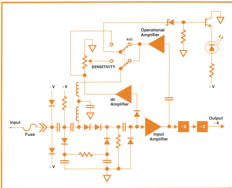
Fig. 5. Input attenuator may be controlled manually or automatically. Usually automatic sensitivity control is better for noisy signals; manual control is better for amplitude-modulated signals.
