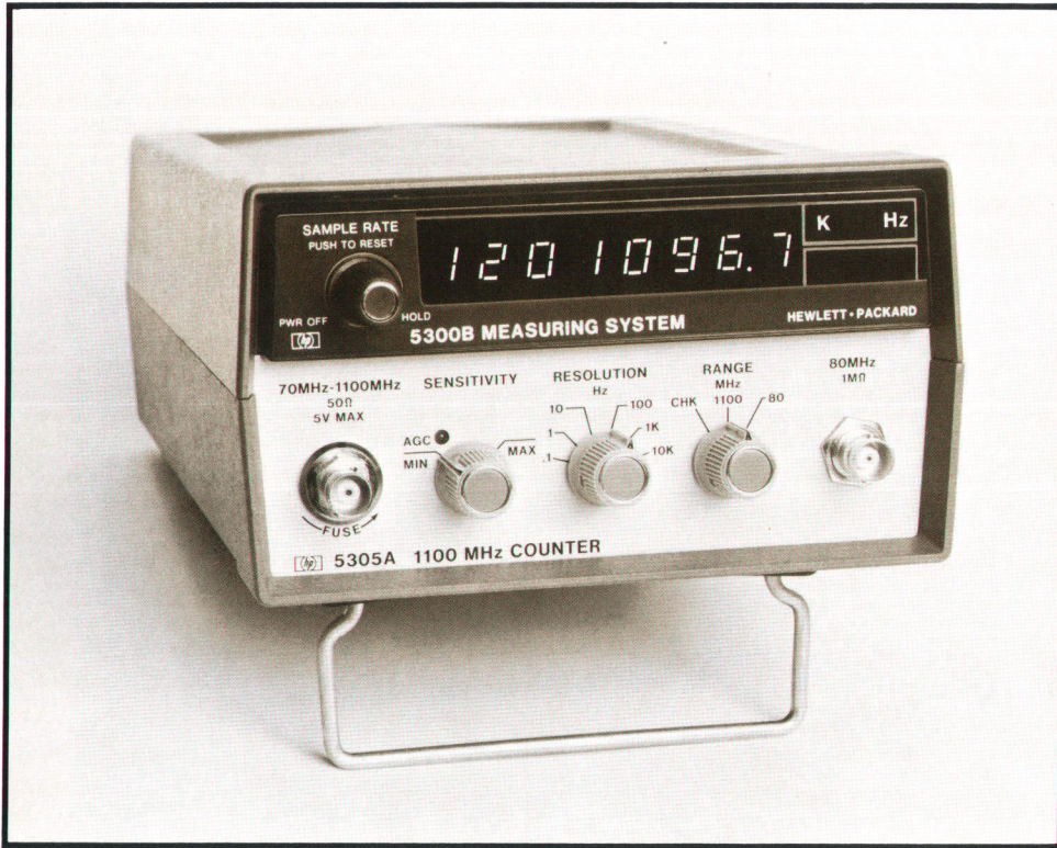
Fig. 1. The new Model 5305A 1100-MHz Frequency Counter (lower module) is shown here with the eight-digit Model 5300B mainframe (upper module). Insertion of a battery pack between the two modules makes the counter completely portable for checking mobile communications systems.
