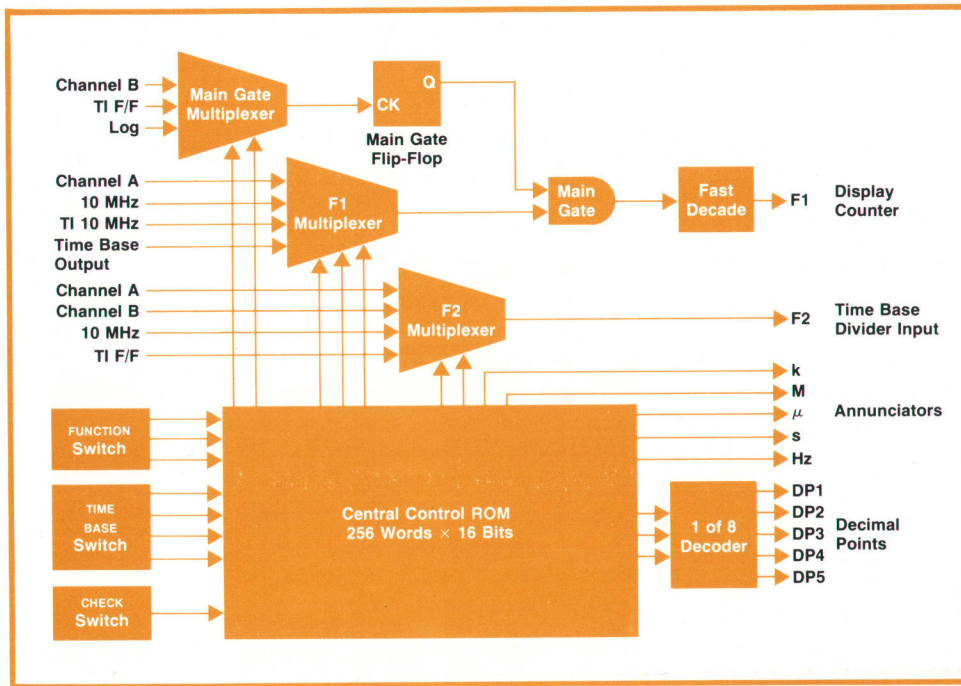
Fig. 2. 5308A function control circuit. Central control ROM made possible much of the new capability of the 5308A, including autoranging and time interval averaging.
