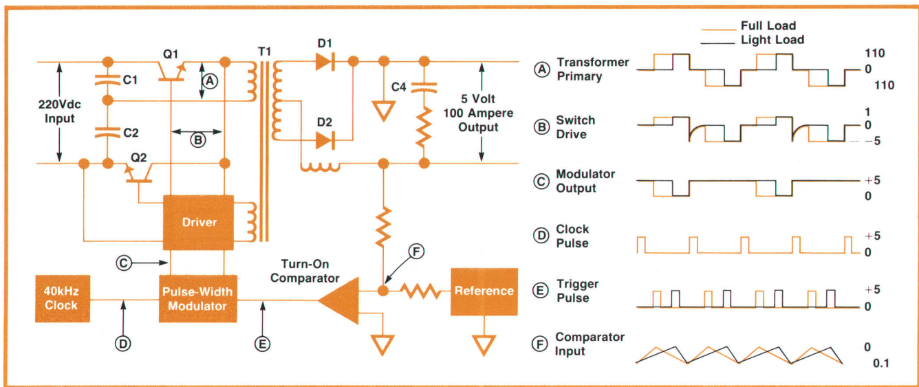
Fig. 6. Switching regulator circuit operates at 20 kHz, a repetition rate that is an optimum compromise with respect to cost, size, dissipation, parts availability, and acoustic noise. The colored waveforms show full-load operation. The black waveforms are typical of lightly loaded operation.
