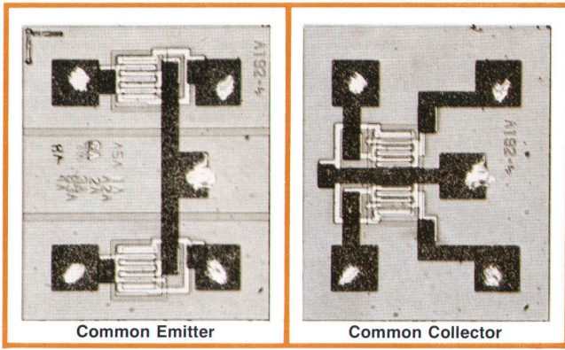
Fig. 6. Special dual-transistor chips, made by a new 5-GHz transistor process, are used in the high-speed binary in the 1100-MHz front end.
