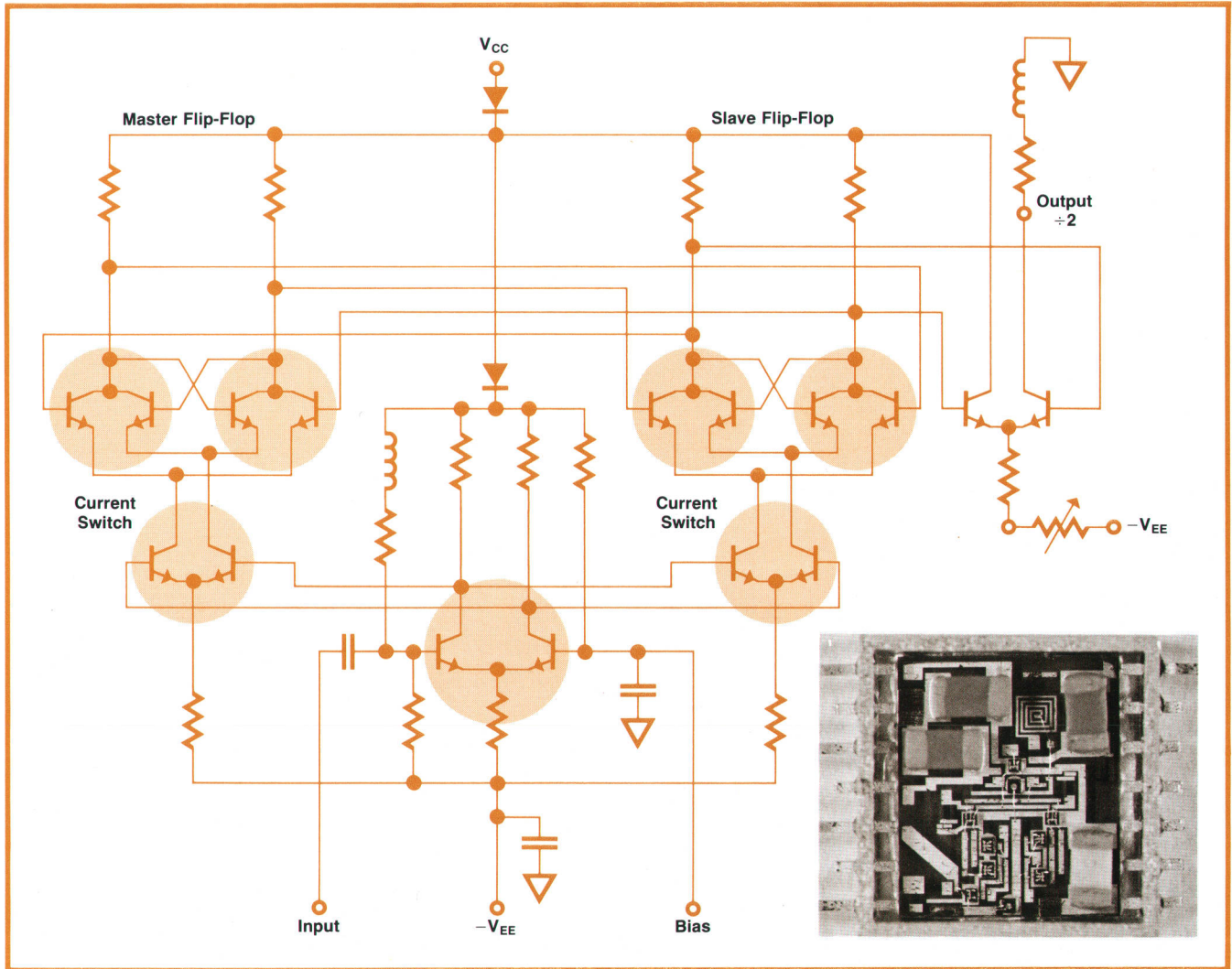
Fig. 7. High-speed binary is a master-slave flip-flop divide-by-two circuit.
