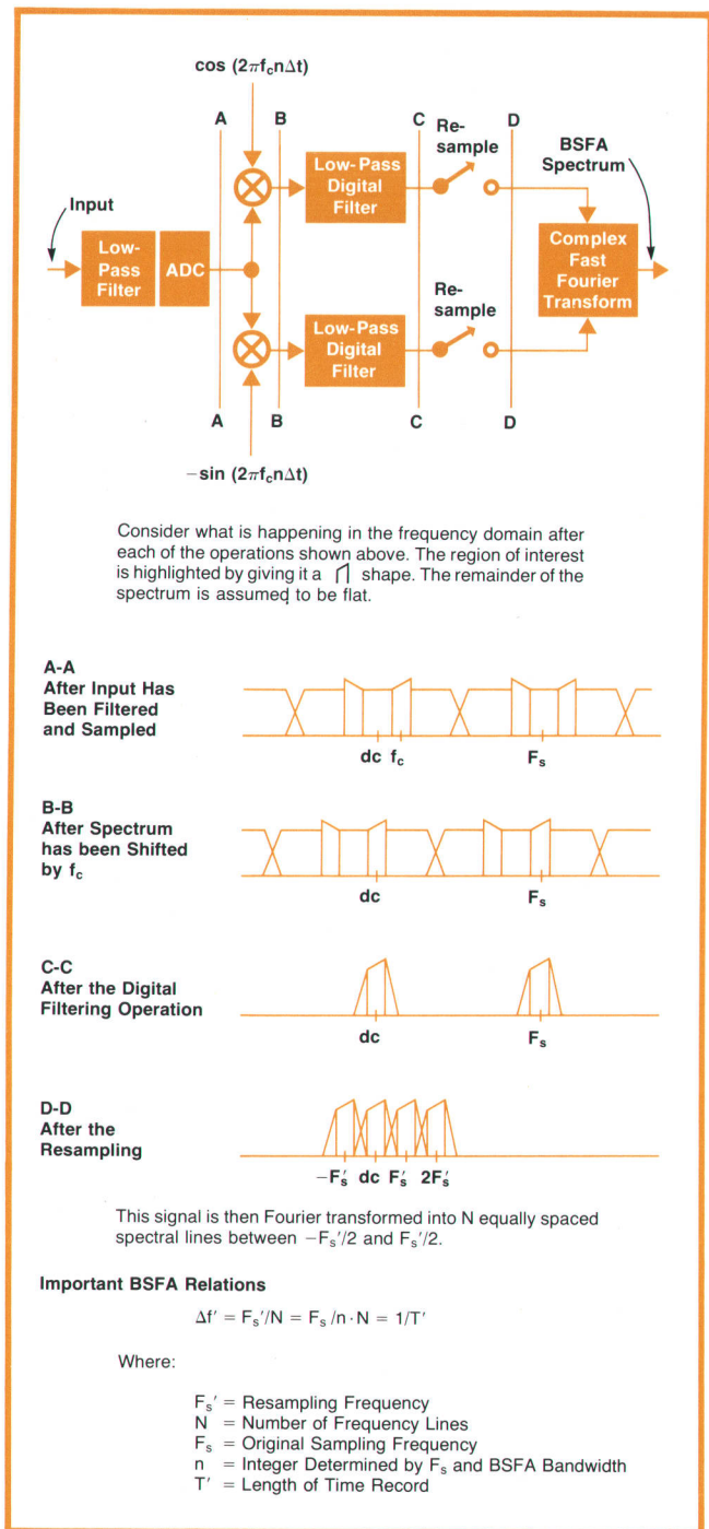
Fig. 5. BSFA signal flow. A frequency shift by f_c centers the analysis band on the frequency of interest and digital filtering removes information outside the band of interest.
