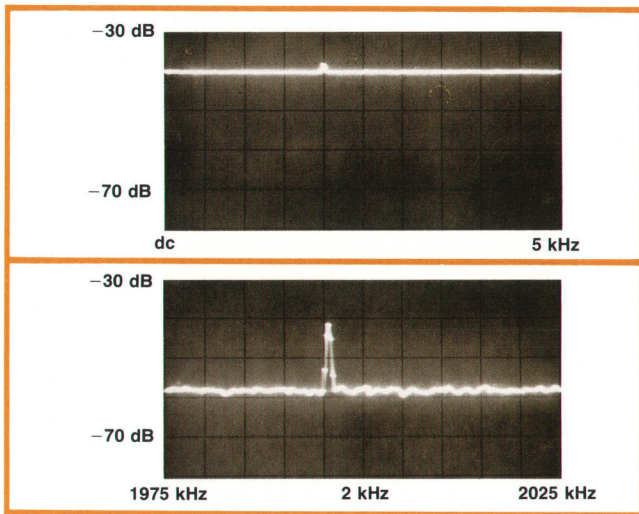
Fig. 2. In the baseband spectrum of a sine wave buried in white noise the sine wave appears only 2 dB above the noise after 10 000 averages. In the BSFA spectrum after only 100 000 averages, the sine wave is 17 dB above the noise and consequently is much more detectable. BSFA's 100 × improvement in resolution results in a reduced mean value for the white noise; however, the noise variance is greater because fewer measurements were averaged. The two measurements required the same total time.
