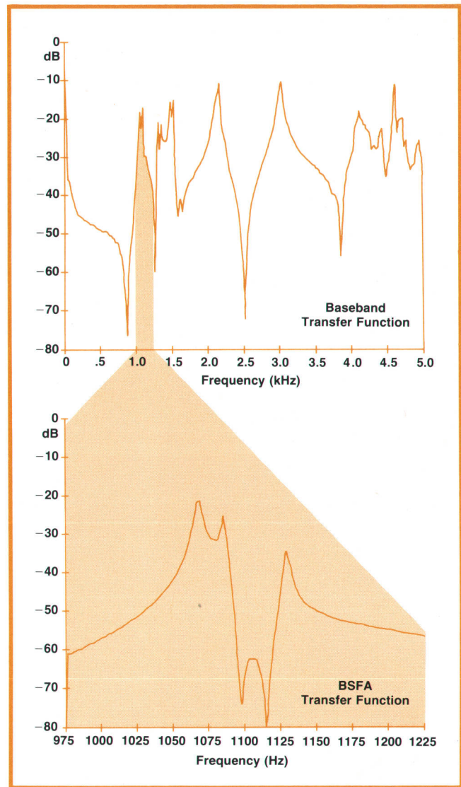
Fig. 3. In this mechanical impedance measurement on a squeaky automobile disc brake rotor, BSFA made possible an accurate determination of the modes of vibration and the damping associated with each mode.
