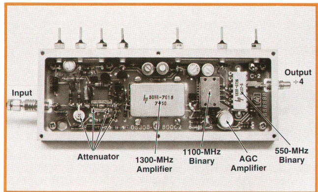
Fig. 3. Completely enclosed high-frequency front end contains an attenuator, a broadband amplifier, a high-speed binary, and a second binary.
