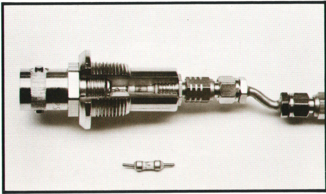
Fig. 4. Special fuse holder in the input BNC connector takes inexpensive, easily obtainable fuses. Fuse protection frees the user from worrying about applying too much power and damaging his expensive front end.
