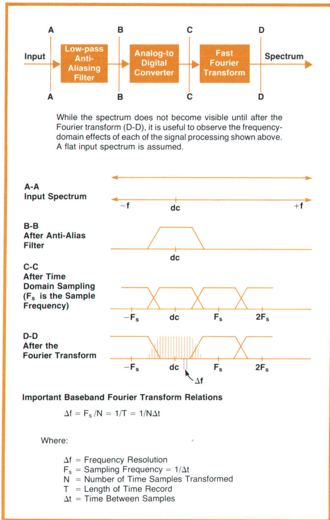
Fig. 4. Signal flow in baseband Fourier Analysis, showing spectra that result from individual processing steps. A flat input spectrum is assumed.
