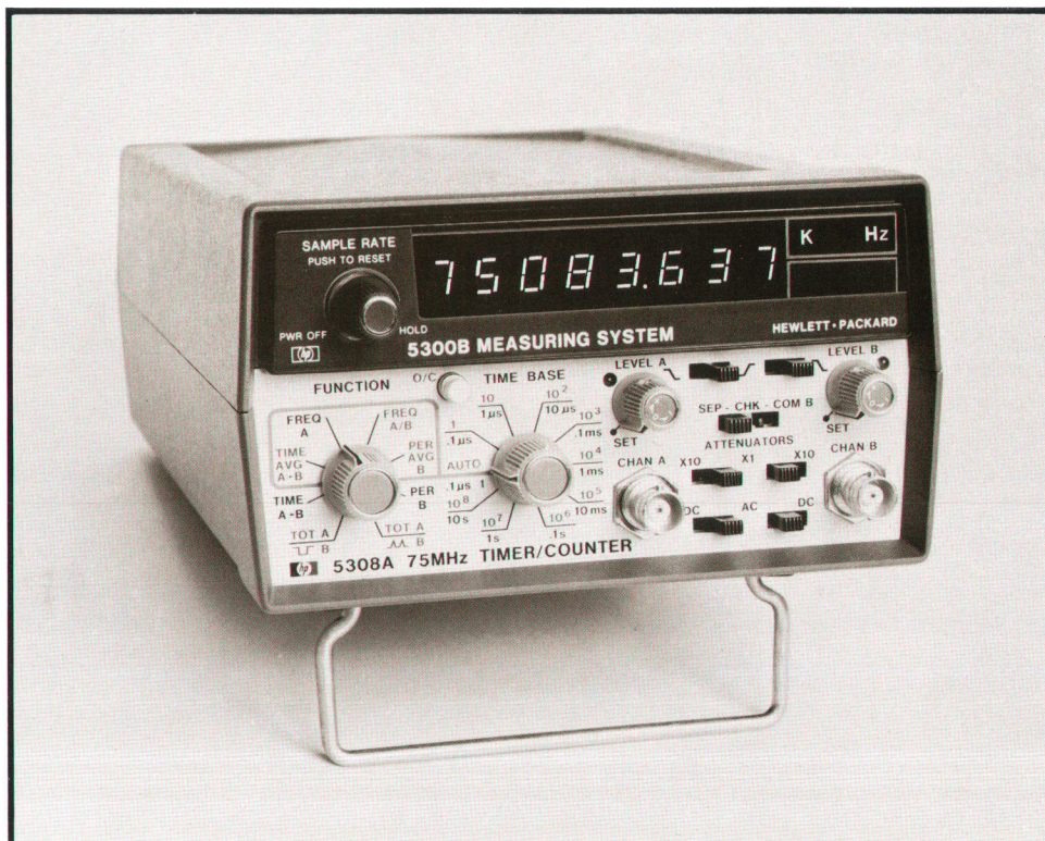
Fig. 1. Model 5308A 75-MHz Timer/Counter (lower module) is an eight-function, eight-digit universal timer and counter that works with the 5300B mainframe. Features include autoranging, trigger lights, and preset trigger levels for logic measurements.
